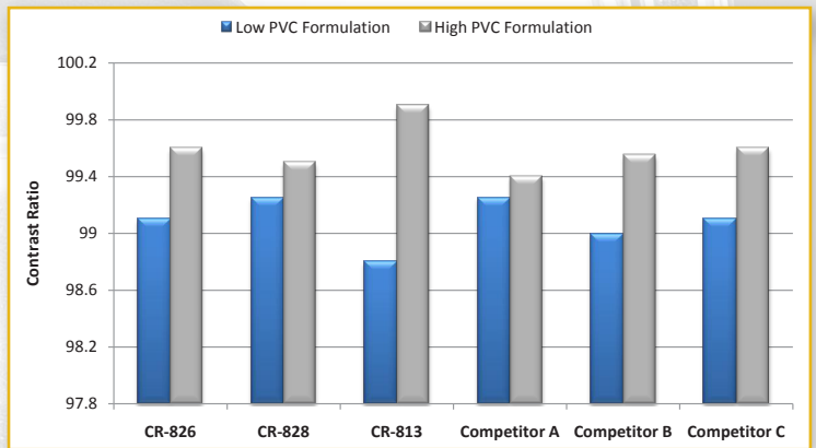
光沢60° - WATERBORNE ACRYLIC EMULSION
