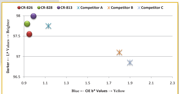
CIE COLOR L* AND b* LOW PVC EMULSION PAINT
